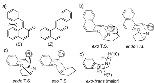
Figure 1. a) Steric repulsion destabilizes the E form. b) Steric repulsion in the exo transition state. c) Steric repulsion in the endo transition state. d) W coupling. T.S. = transition state.
