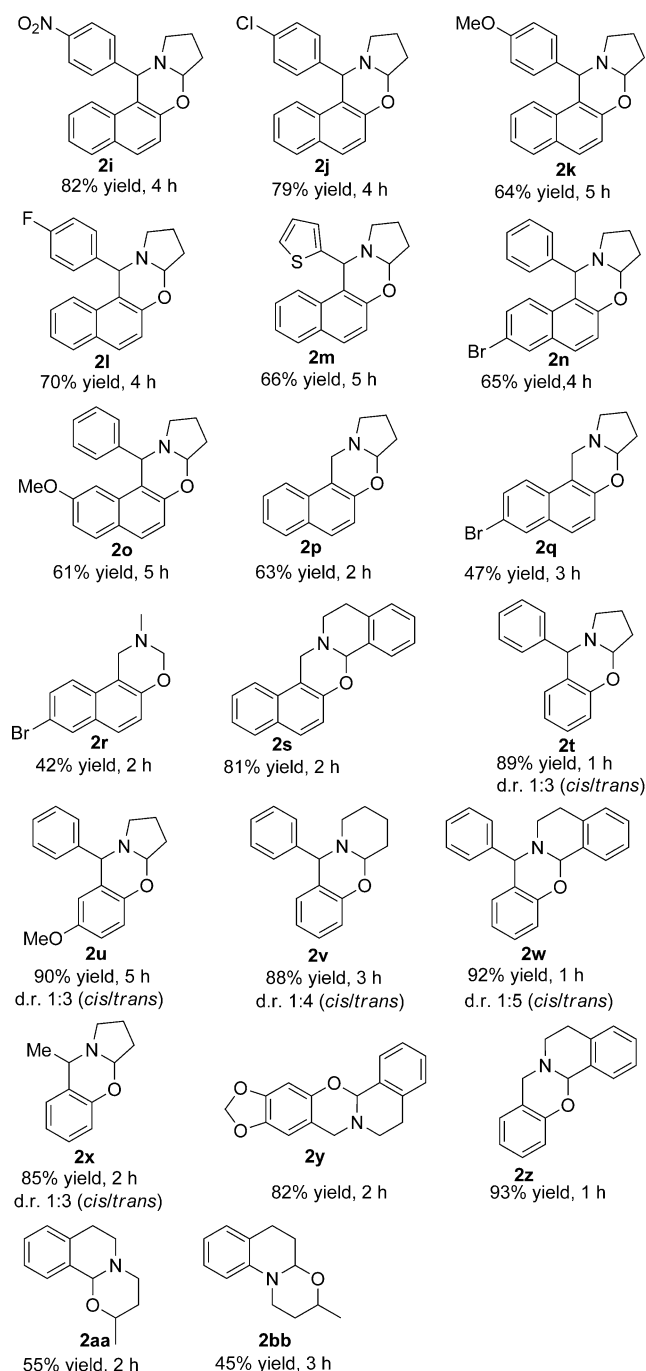
Scheme 2. Substrate scope for the synthesis of 1,3-oxazines. Reaction conditions: 1 (0.2 mmol), Cu(OAc) 2 ·H 2 O (5 mol%), p -xylene (1 mL) at 130 °C. Yields shown are of isolated products. Isomer ratios are not specified where only the trans isomer was observed by NMR spectroscopy.
